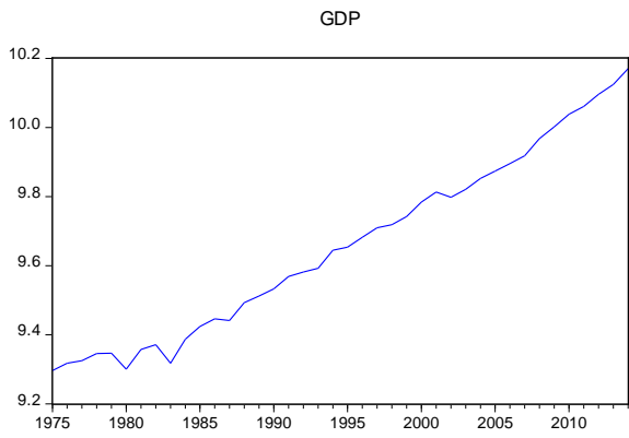
Figure 1 Trends in the transformed variables
