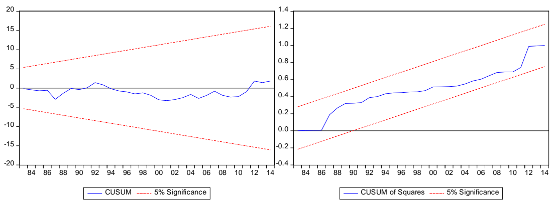
Figure 3 Stability test for model tourist arrivals
