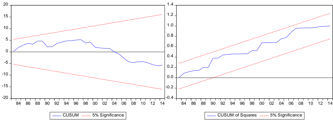
Figure 2 Stability test for model CO 2 emissions
