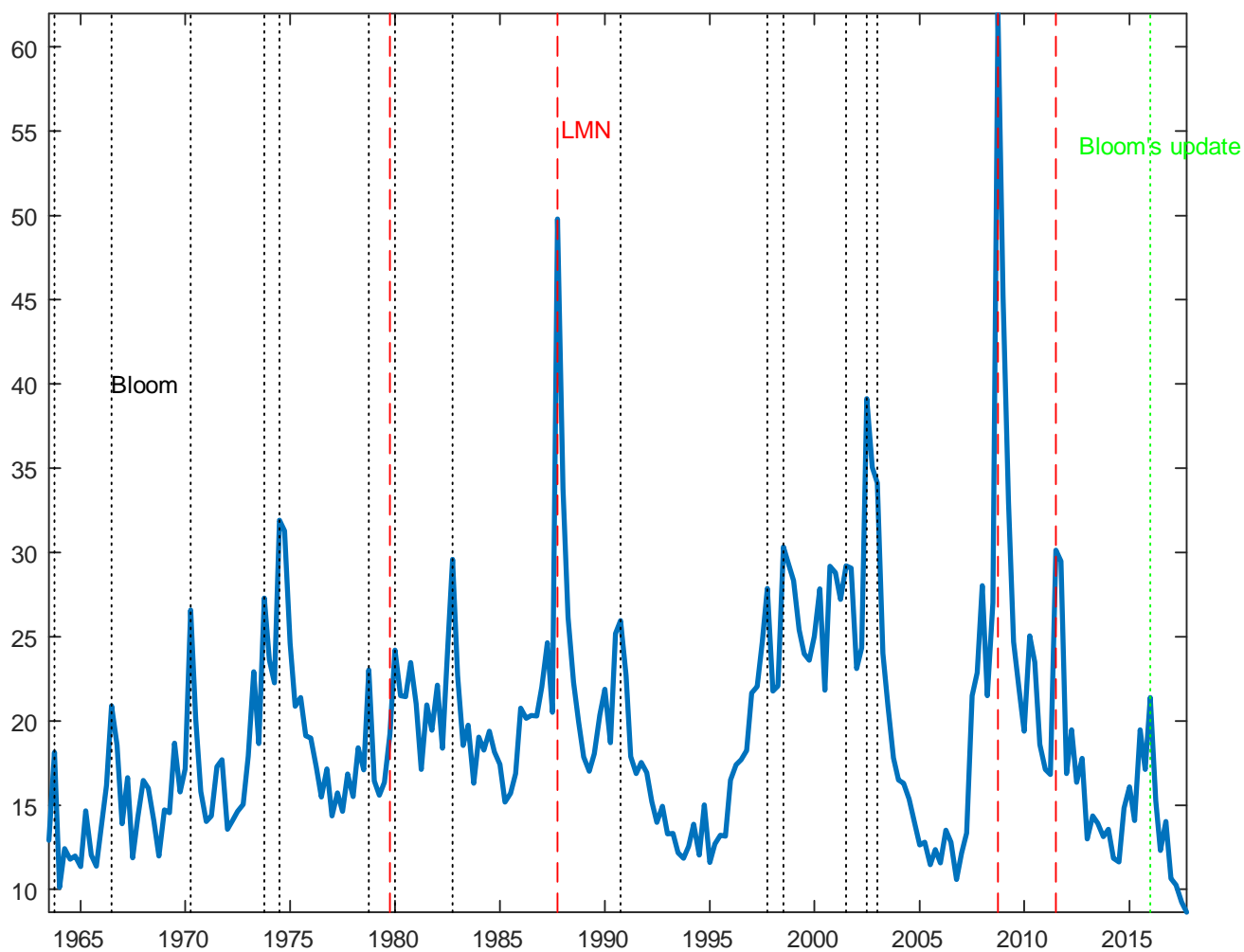
Figure 1: Financial uncertainty: Identified peaks. Vertical lines identify the events used to identify financial uncertainty shocks. The four red lines refer to the events selected by Ludvigson, Ma and Ng (2019). The black lines identify the dates selected by Bloom (2009). The green line refers to the 2016 increase not covered in Bloom (2009). Further details are reported in Table 1.
