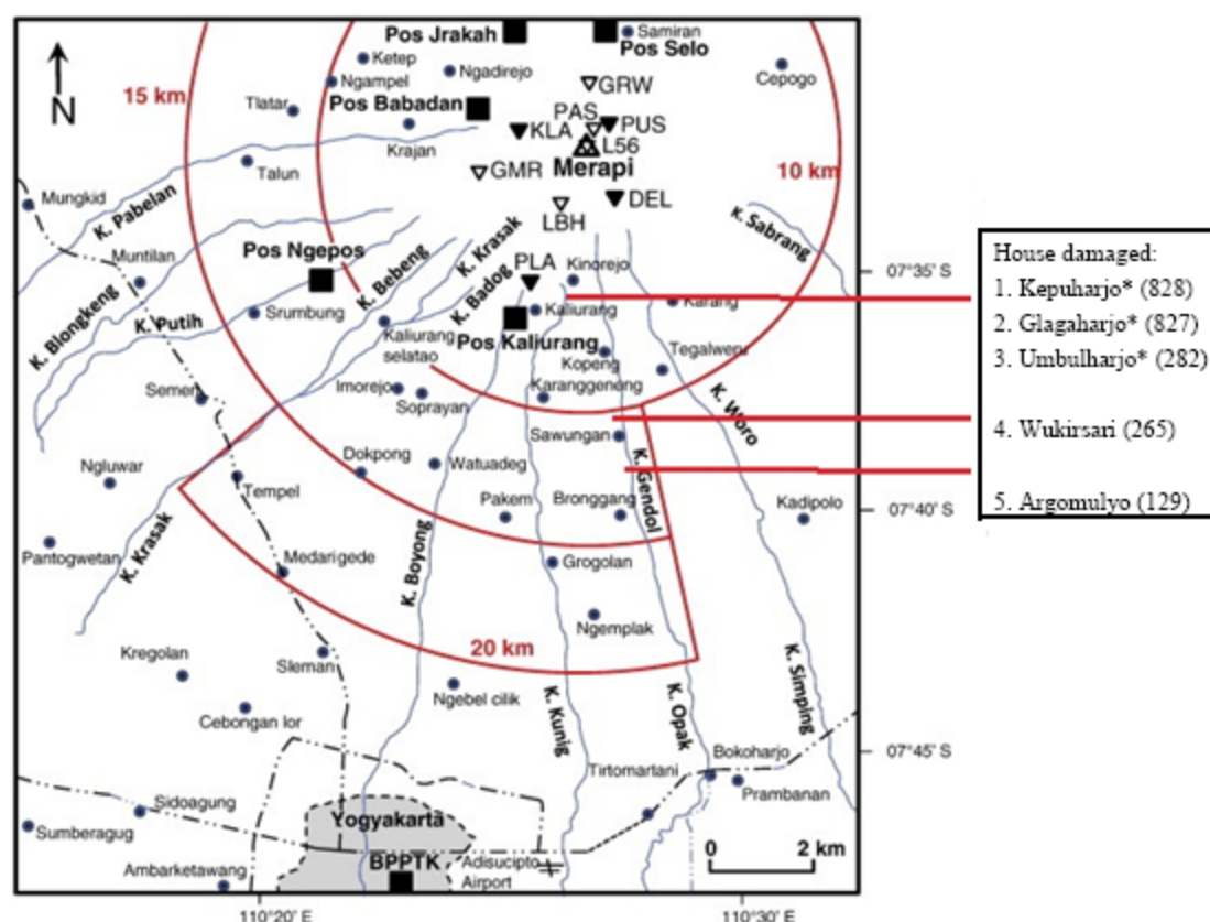
Figure 2. Number of houses damaged in the Cangkringan subdistrict due to the Merapi eruptions in 2010.
