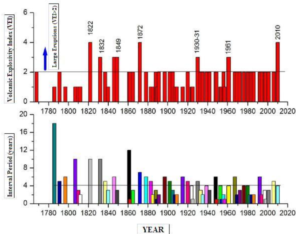
Figure 1. The history of Merapi eruptions.
