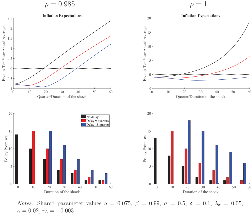
Figure 7: Optimal Policy: Is it worth the wait?
