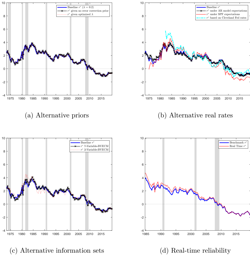
Figure 3: Robustness of r^* estimates
