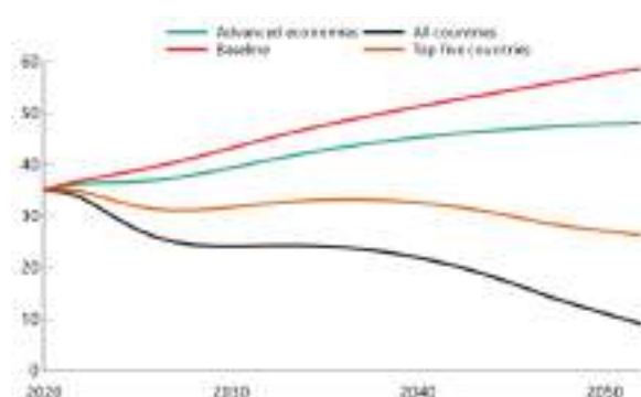
Global CO2 emissions (gigatons of CO2)
