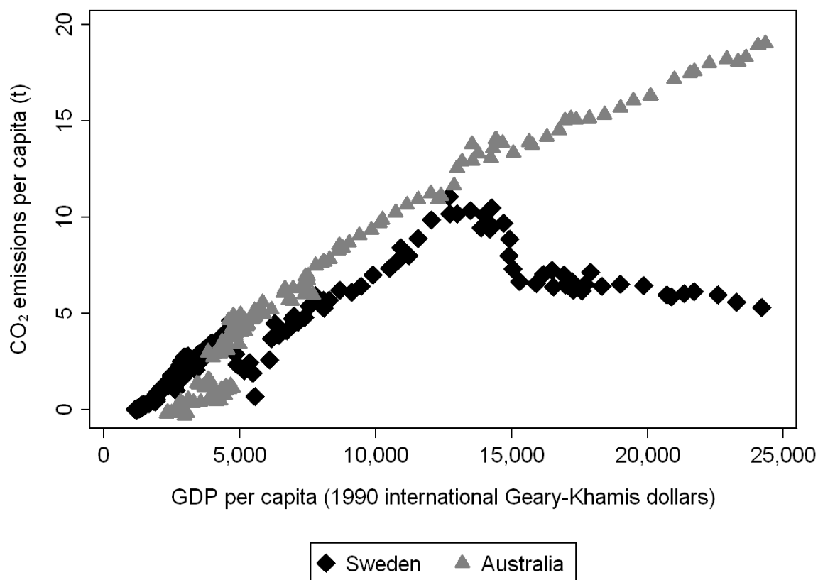
Figure 1 CO 2 emissions-income paths for Sweden and Australia, 1851-2006. Emissions are those from fossil fuel use. Emissions data source: 1851-1959: Boden et al. (2009); 1960-2006: International Energy Agency [IEA] (2009a). GDP and population data source: Maddison (2009).
