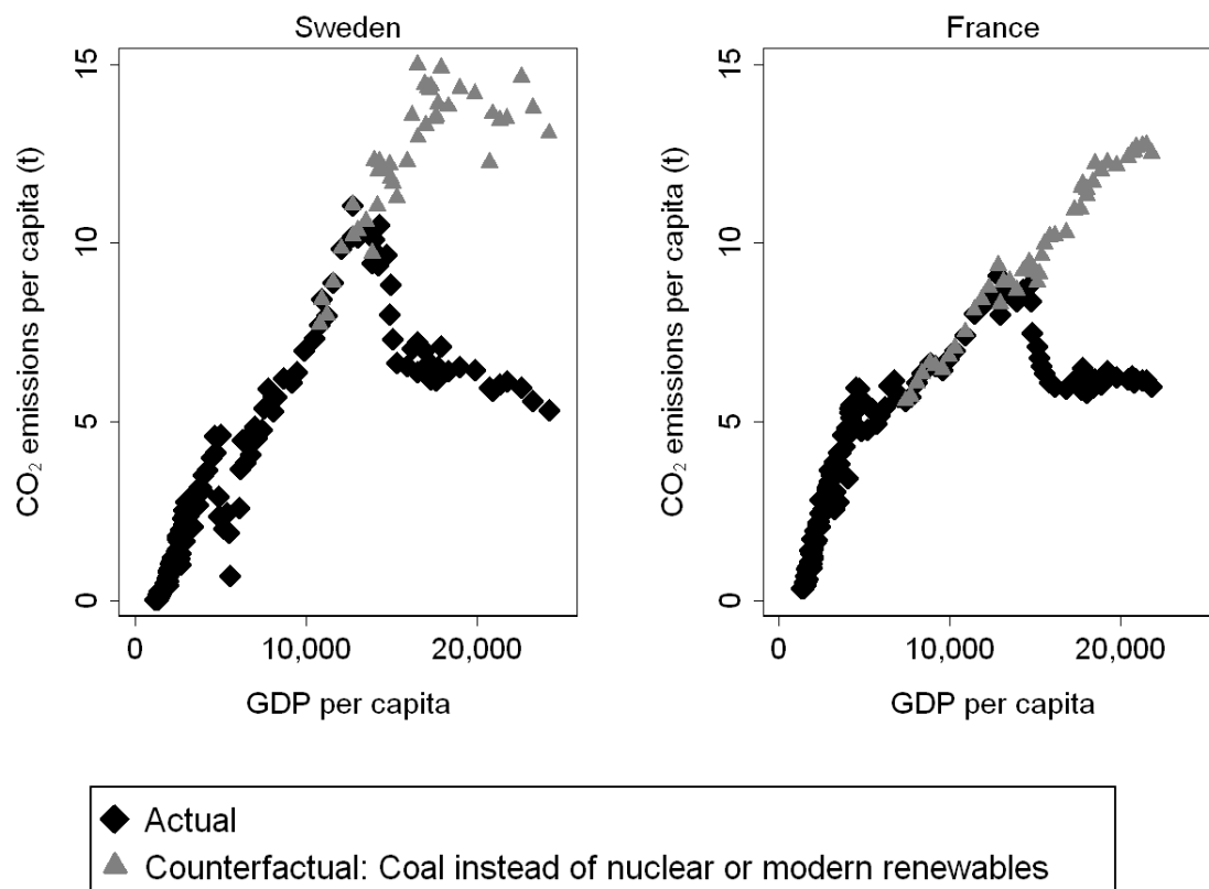
Figure 2 Actual and “coal instead of nuclear and modern renewables” counterfactual CO 2 emissions-income paths for Sweden and France, 1839-2006. Emissions are those from fossil fuel use. GDP per capita is in 1990 international Geary-Khamis dollars. The counterfactual is constructed assuming that electricity generated from nuclear power and modern renewables was instead generated from coal sources that produce 0.90372 kilograms of CO 2 per kilowatt hour of electricity (the OECD average for the period 1992-2006; source: IEA 2009c). Emissions data source: 1851-1959: Boden et al. (2009); 1960-2006: IEA (2009a). GDP and population data source: Maddison (2009). Electricity data source: IEA (2009b).
