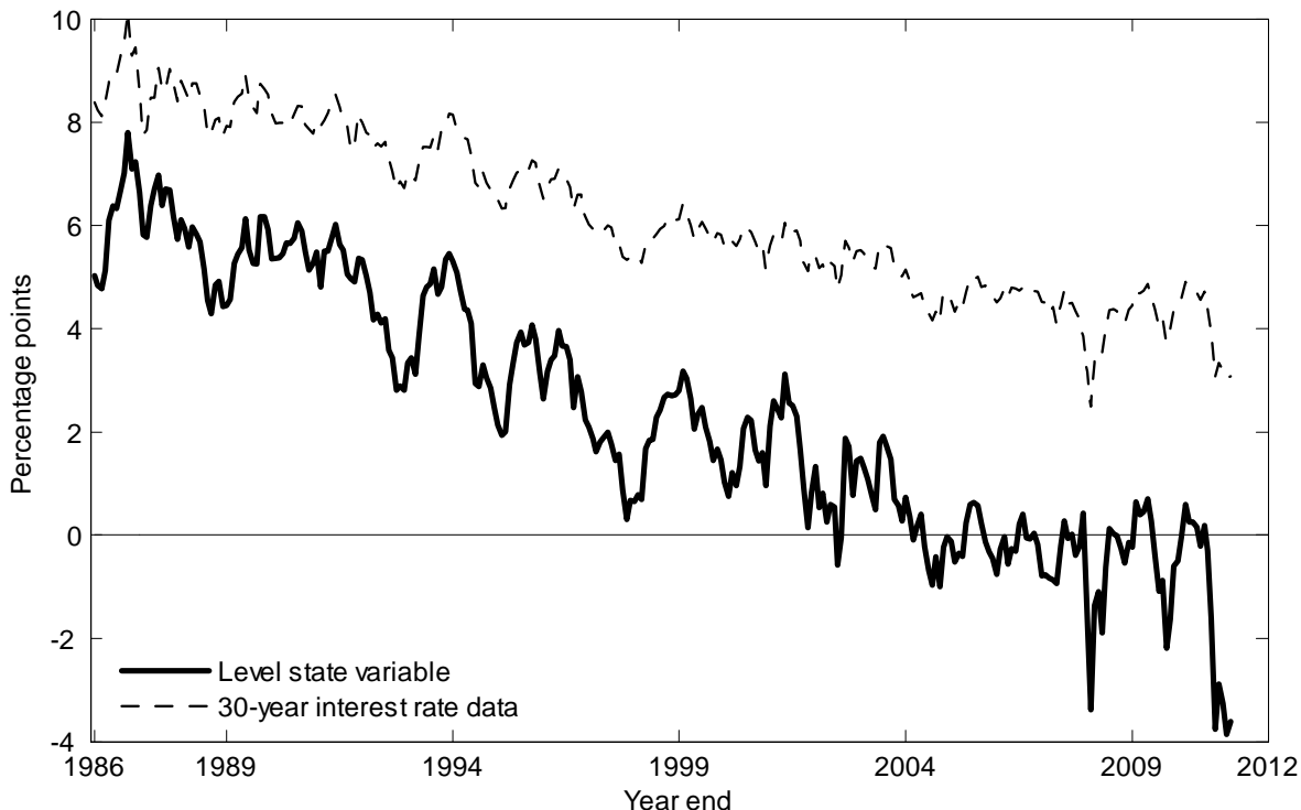
Figure 5: The 30-year interest rate data and estimates of the ZLB-GATSM(2) Level state variable s_1(t) .
