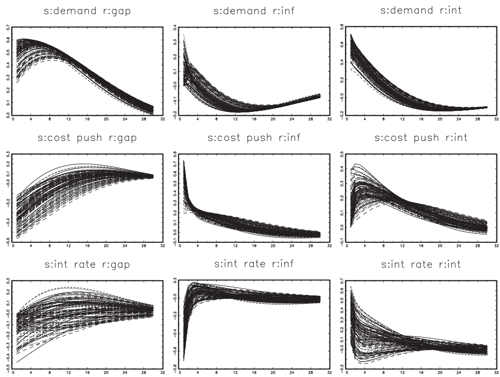
Figure 1: 1000 Impulse Responses Found with the Sign Restrictions of Table 2
