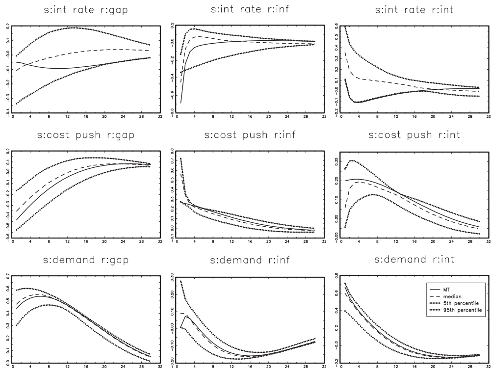
Figure 2: Impulse Responses for Macro Model: Median, MT and 5,95 Percentiles
