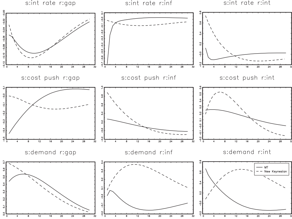
Figure 3: Comparison of the impulse responses of the small macro model (MT method - solid line), and a New Keynesian model (dashed line).
