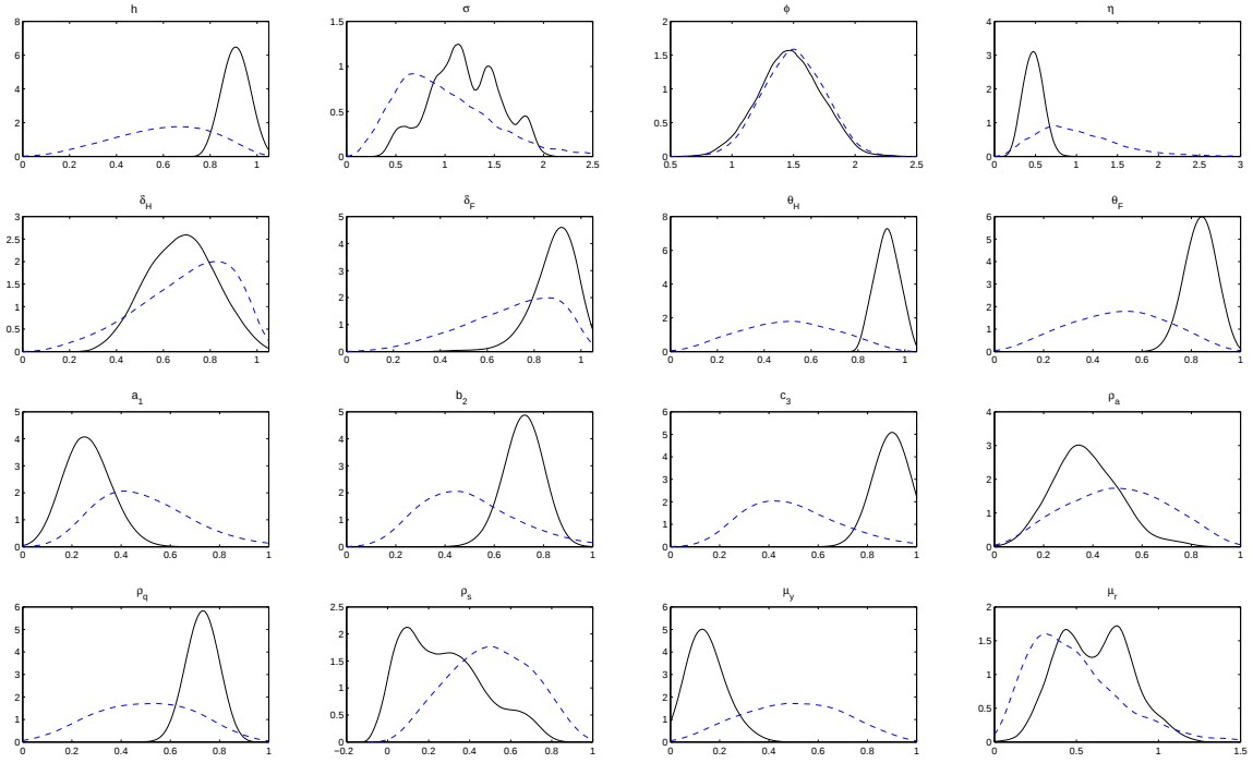
Fig. 2. Posterior distribution of key parameters: Canada. Prior (dashed) and Posterior (solid).
