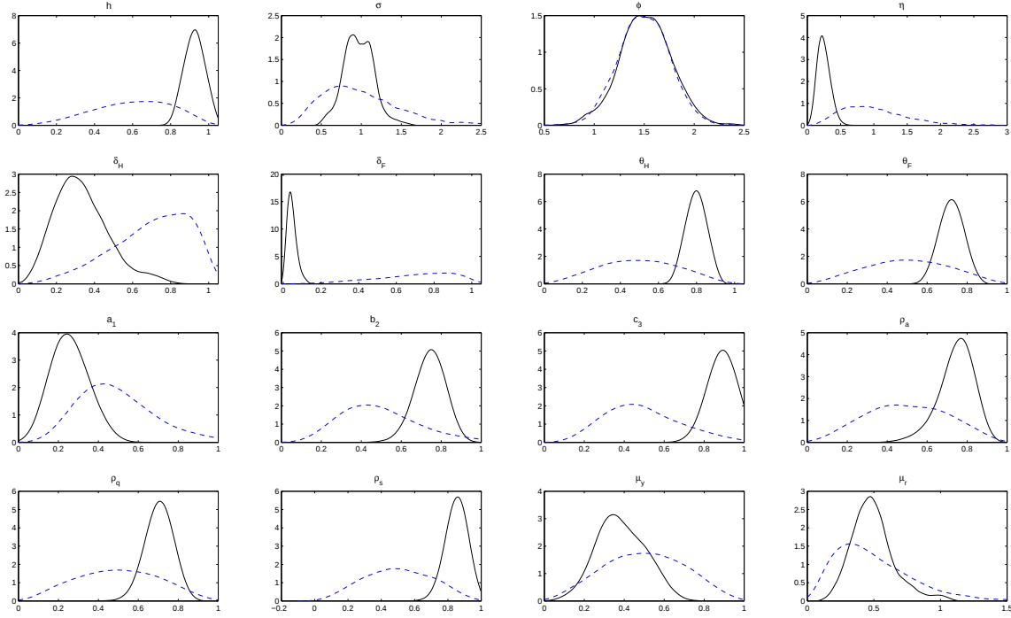
Fig. 1. Posterior distribution of key parameters: Australia. Prior (dashed) and Posterior (solid).
