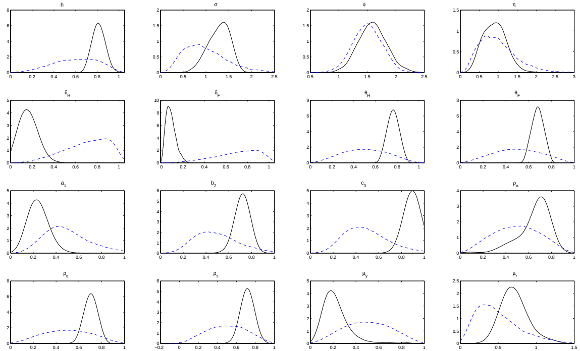
Fig. 3. Posterior distribution of key parameters: New Zealand. Prior (dashed) and Posterior (solid).
